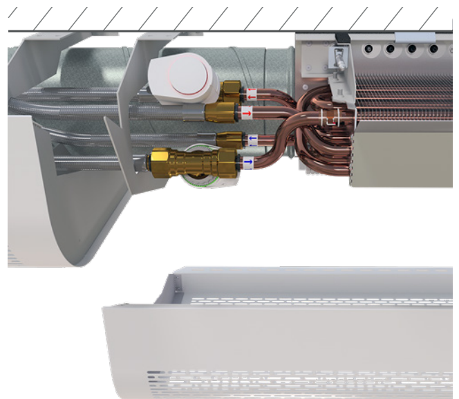
Picture 8. Plafond XD with Cover Clyp in series.
