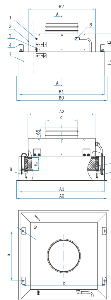
AFV-8B/F/_R_-V (racord vertical)
